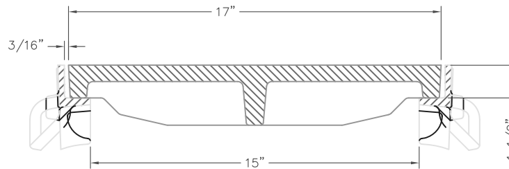
R-4990-EX TYPE "E" VENTED LID WITH TYPE "B" FRAME TYPICAL SECTION (SCALE: 1/4"=1")
